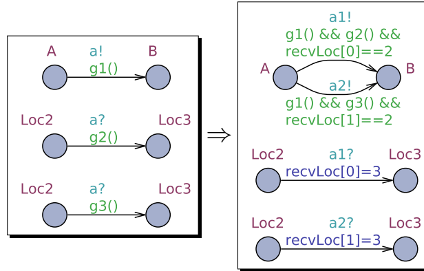
Figure 20: Extended case of a one-to-any channel synchronization (only two here) and its translation to a broadcast channel synchronization.
