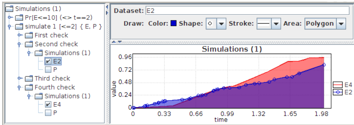
Figure 18: Visual data comparison in the Plot Composer.
