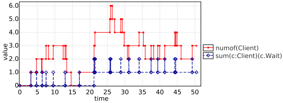
Figure 13: Plot of the number of waiting and total number of clients from the query: simulate 1 [≤50] { numOf(Client), sum(c:Client)(c.Wait) }
