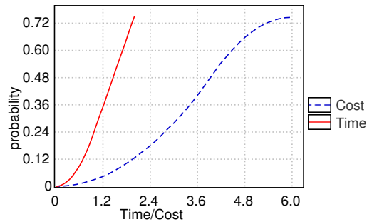
Figure 4: Cumulative probabilities for time and Cost -bounded reachability of T_3 .
