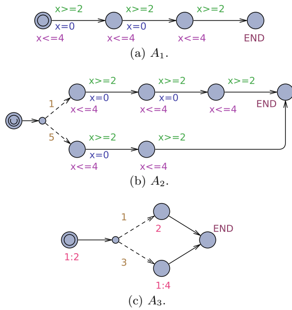
Figure 1: Three stochastic timed automata.
