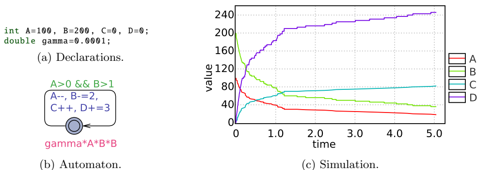
Figure 24: Stochastic model and its behavior.
