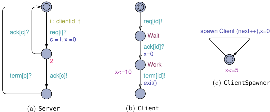
Figure 12: Modeling a server with dynamic spawning
