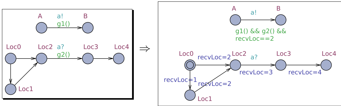
Figure 19: Basic case of a one-to-one channel synchronization and its translation to a broadcast channel synchronization.
