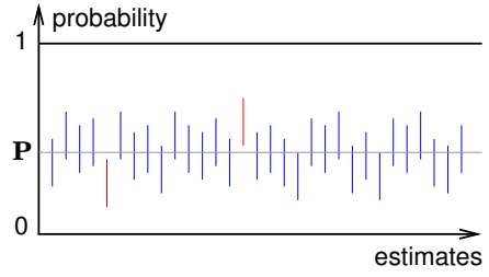
Figure 7: True probability \mathbf{P} and confidence intervals.
