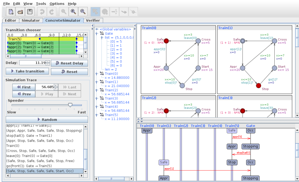
Figure 15: The concrete simulator in UPPAAL.
