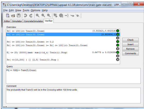
(a) The Verifier of UPPAAL SMC
