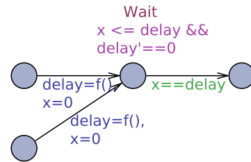
Figure 22: Pattern for custom delay distributions.
