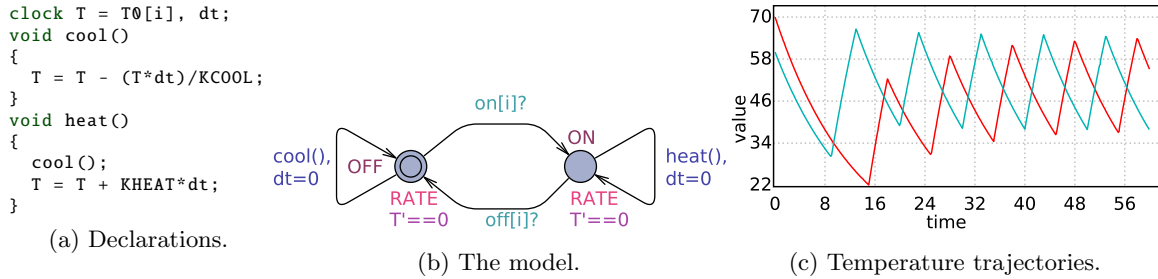
Figure 28: The temperature of a heated room with a manual discretization using a high exponential rate RATE .
