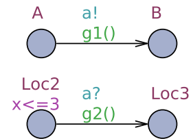
Figure 21: Problematic case where the translation to broadcast channel is not possible.
