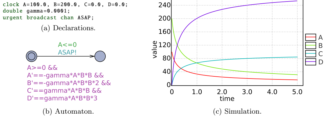
Figure 26: Dynamical model and its behavior.
