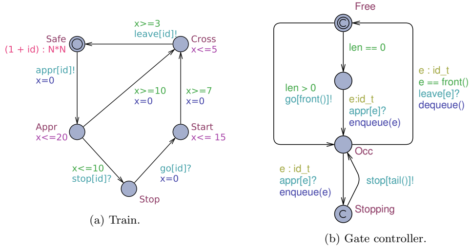
Figure 5: Templates for the train-gate example.
