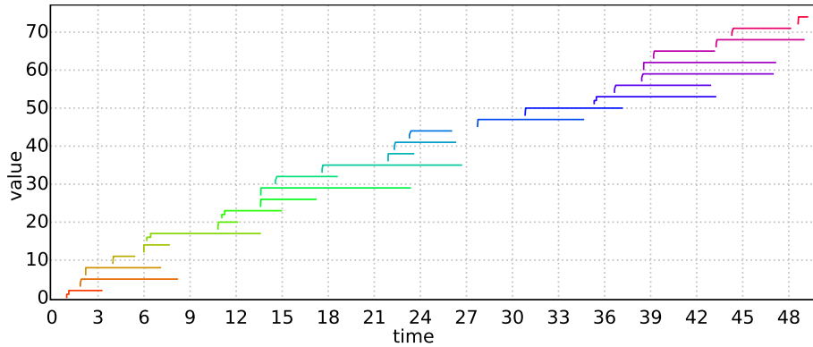
Figure 14: Life span of each client from the query: simulate 1 [≤50] { numOf(Client), sum(c:Client)(c.Wait) }
