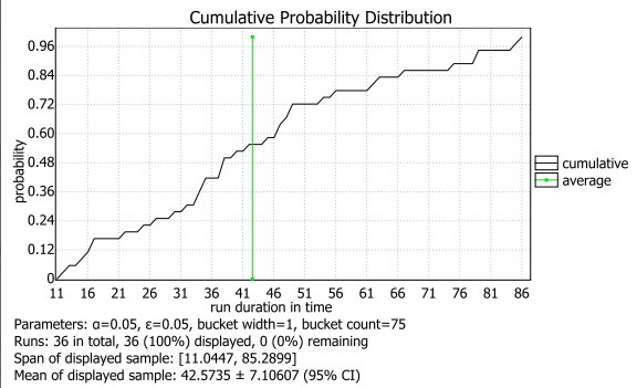
(b) The cumulative probability distribution of \text{Pr}[\leq \Gamma] (\triangleleft \text{Train}(5).\text{Cross}) .
