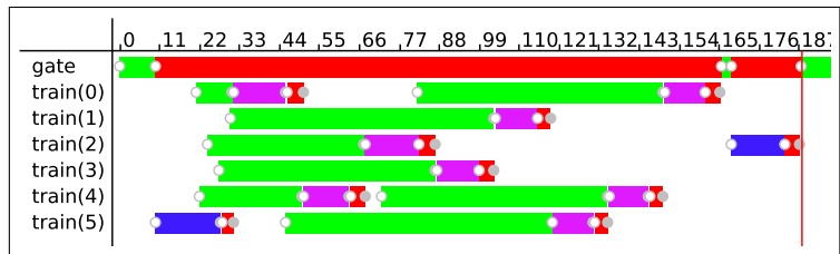
(b) Trace visualization in Concrete Simulator.
