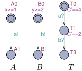
Figure 3: An NSTA, (A|B|T) .
