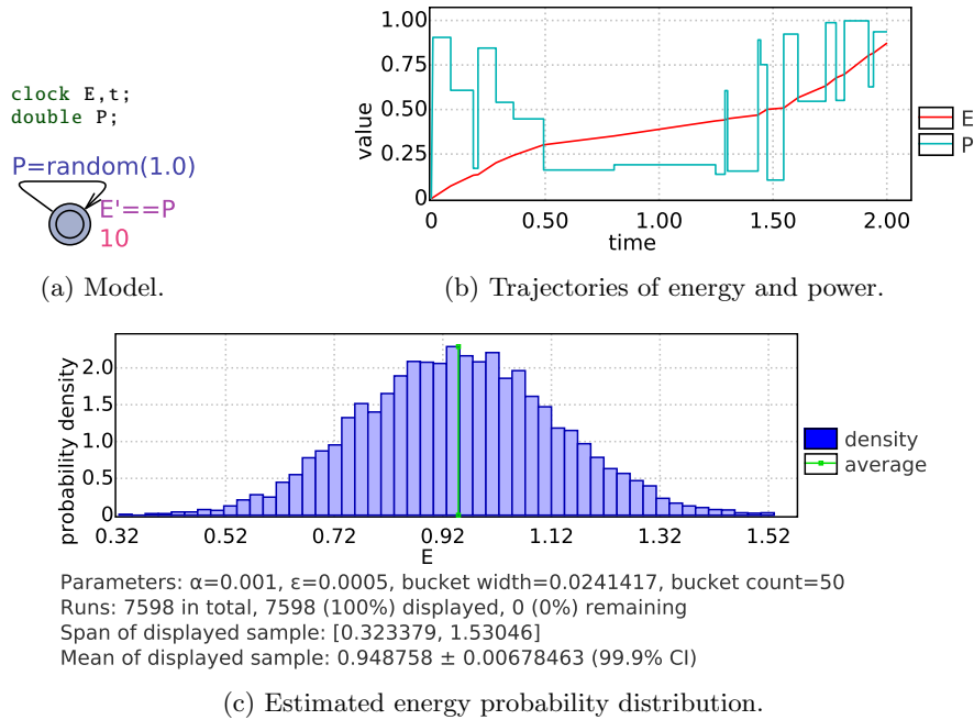
Figure 27: Cost estimation in terms of energy.
