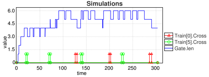
Figure 6: Visualizing the gate length and when Train(0) and Train(5) cross on one random run.
