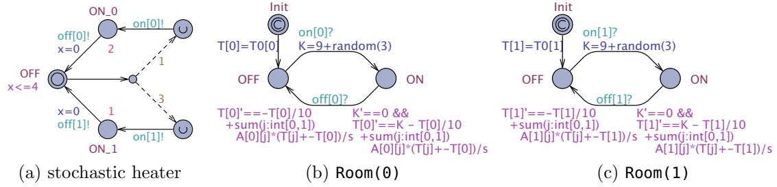
Figure 10: A simple two room example with an autonomous heater
