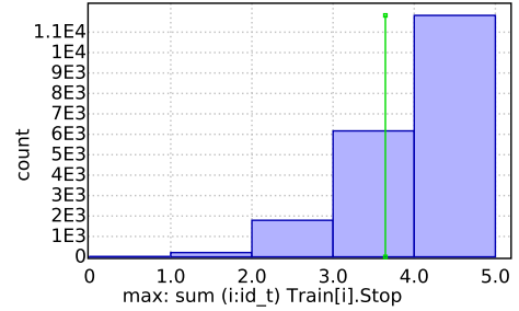
Figure 9: Frequency histogram of maximum number of trains stopped within 20 time-units.
